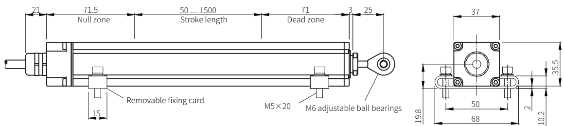
Axial outlet, Straight out cable
